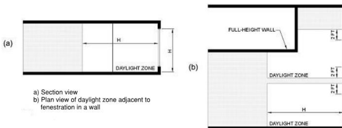
FIGURE C405.2.3.2 SIDELIT ZONE
