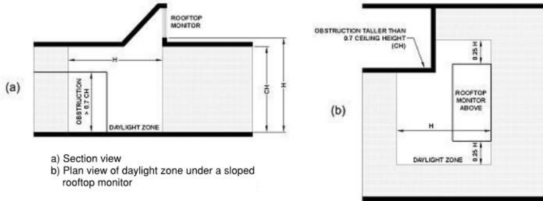
FIGURE C405.2.3.3(3) DAYLIGHT ZONE UNDER A SLOPED ROOFTOP MONITOR
