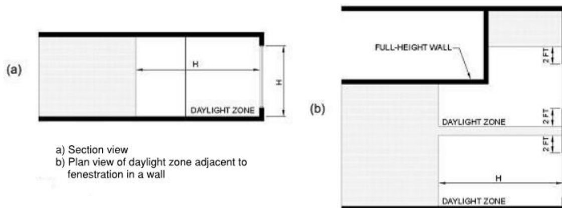
FIGURE C405.2.3.2 SIDELIT ZONE
