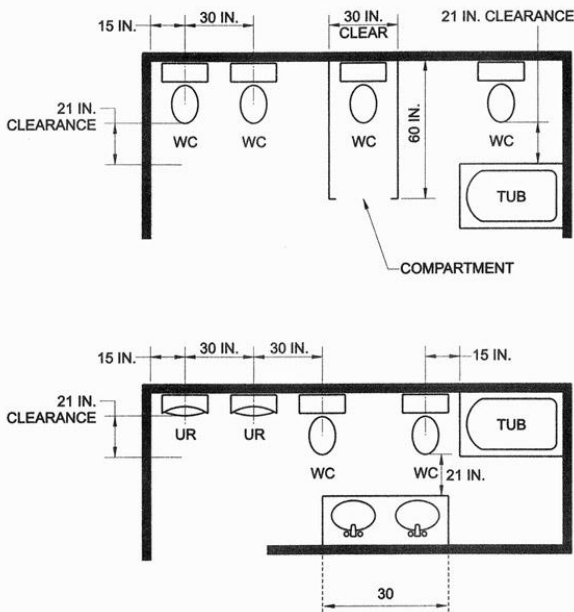
[FIGURE 405.3.1 FIXTURE CLEARANCE] For SI: 1 inch = 25.4 mm
