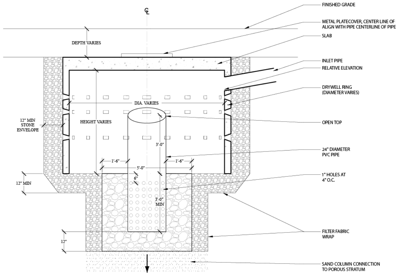
FIGURE 1114.2.3(2) DETAIL OF DRYWELL WITH SAND COLUMN
