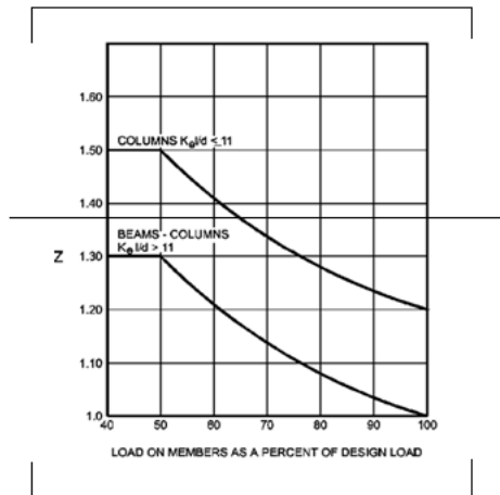
[FIGURE 721.6.3(1)] [LOAD FIGURE]
