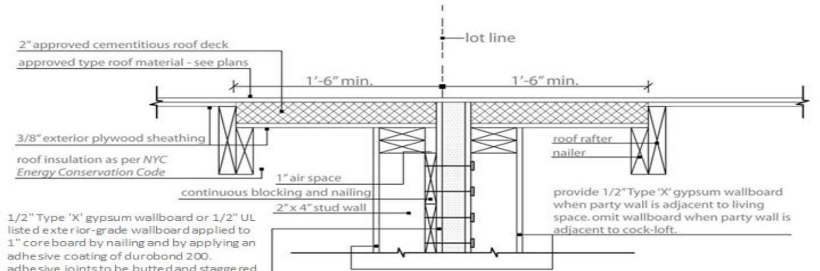
section through two hour rated party wall with sloped or roofs at same level (no projection)
