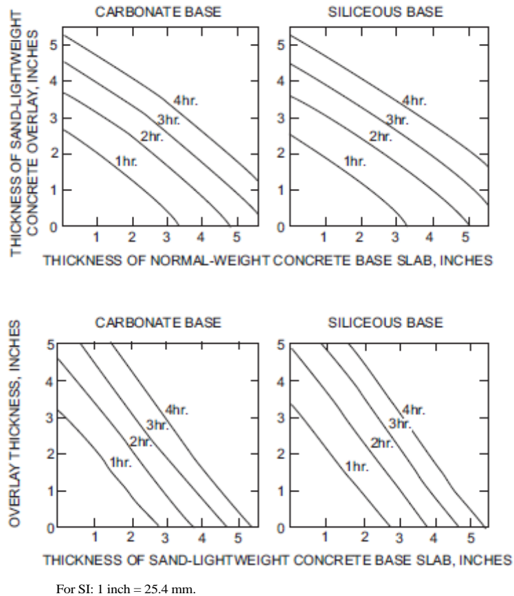
FIGURE [721.2.2.2] 722.2.2.2 FIRE-RESISTANCE RATINGS FOR TWO-COURSE CONCRETE FLOORS
