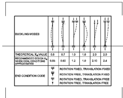
[FIGURE 721.6.3(2)] [EFFECTIVE LENGTH FACTORS]
