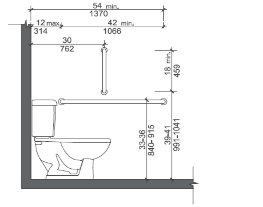
FIGURE 1107.2.2.7.3.1 SIDEWALL GRAB BAR LOCATION
