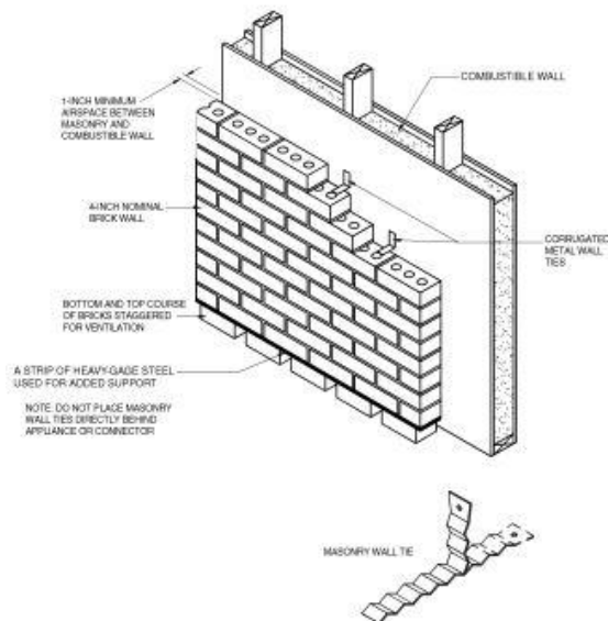
FIGURE 308.2(2) WALL PROTECTOR CLEARANCE REDUCTION SYSTEM
