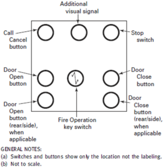
Fig. 2.27.3.3.7 Panel Layout
