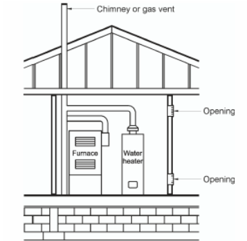
FIGURE 304.5.3 ALL AIR FROM INSIDE THE BUILDING (see Section 304.5.3)
