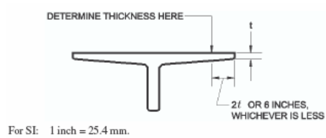
FIGURE 721.2.2.1.2 DETERMINATION OF SLAB THICKNESS FOR SLOPING SOFFITS
