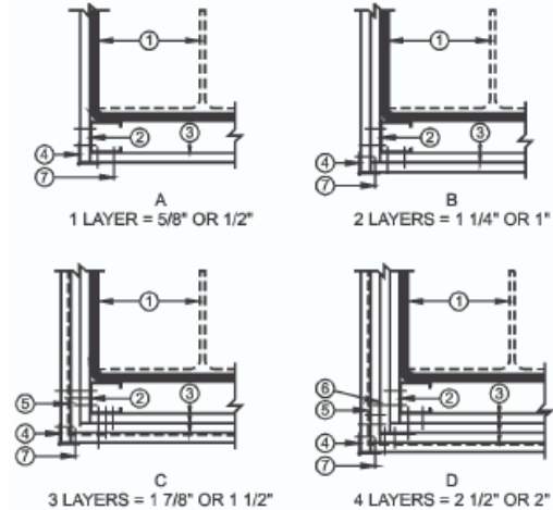
FIGURE 721.5.1(3) GYPSON WALLBOARD PROTECTED STRUCTURAL STEEL COLUMNS WITH STEEL STUD/SCREW ATTACHMENT SYSTEM
