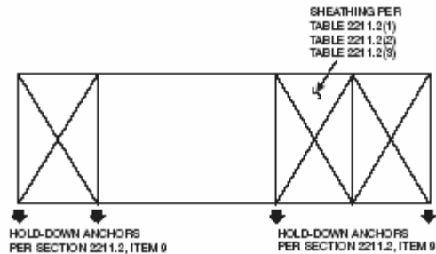
TYPE 1 SHEAR WALL
