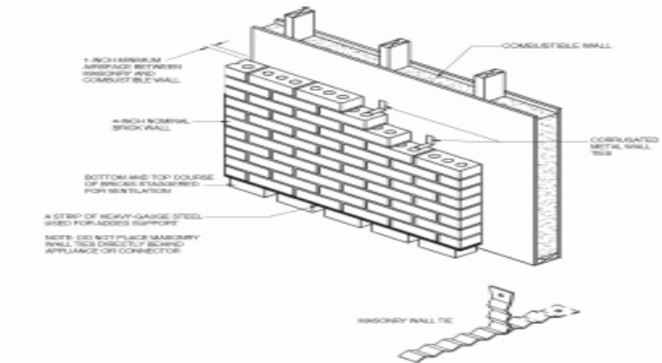
FIGURE 308.2(3) MASONRY CLEARANCE REDUCTION SYSTEM
