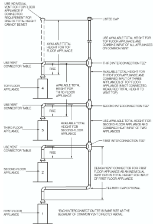
Principles of design of multistory vents using vent connector and common vent design tables (see Sections 504.3.11 through 504.3.17).
