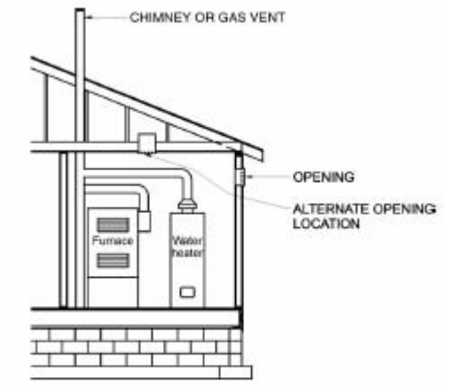
FIGURE 304.6.2 SINGLE COMBUSTION AIR OPENING, ALL AIR FROM THE OUTDOORS (see Section 304.6.2)
