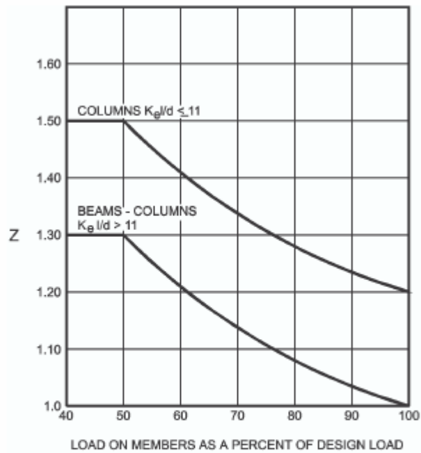
FIGURE 721.6.3(1) LOAD FIGURE
